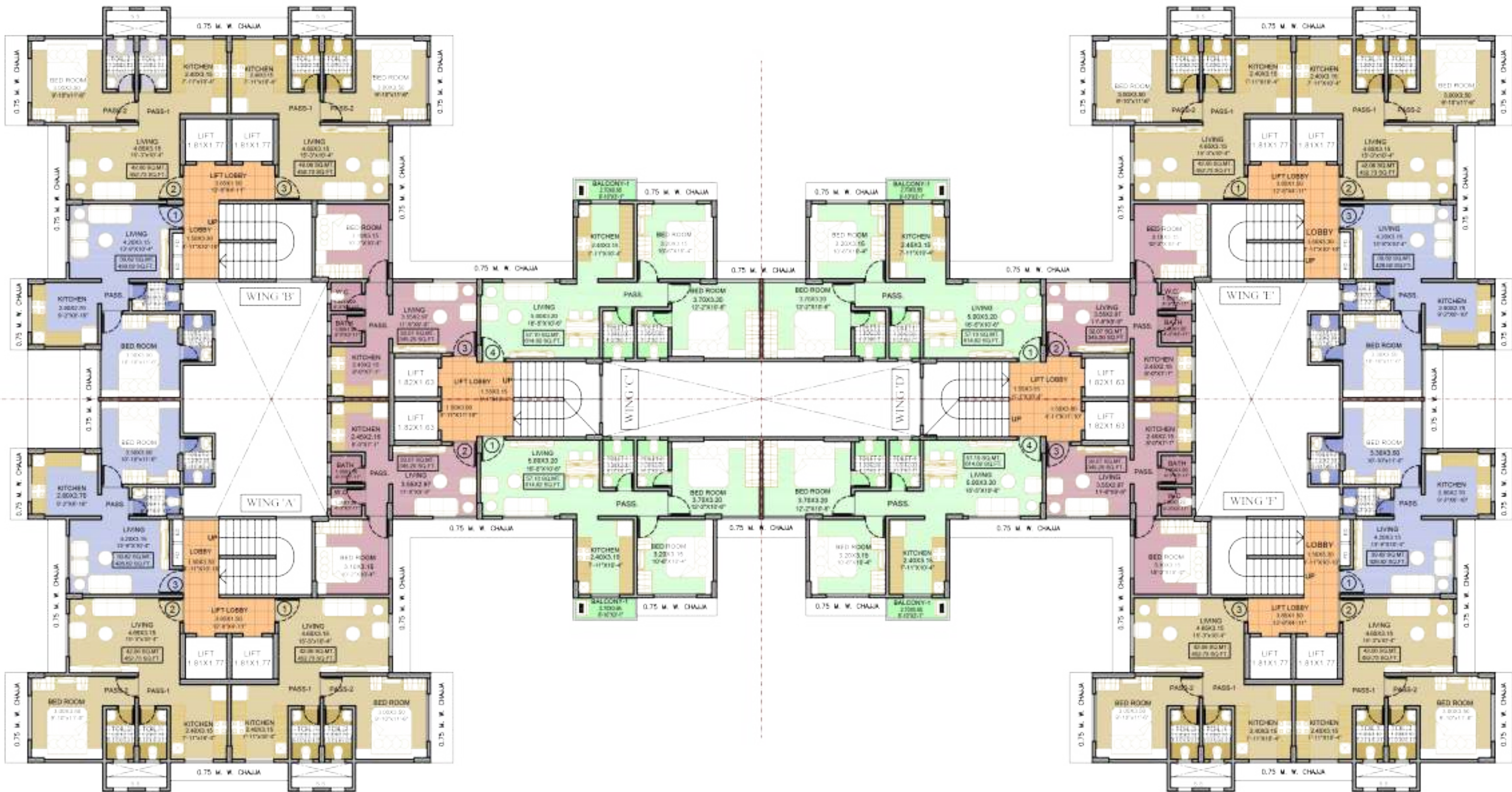
2 to 7 th Floor Plan
